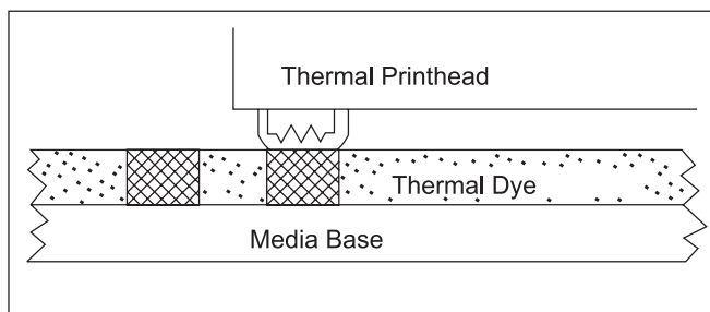
Figure 5. Direct Thermal Printing
